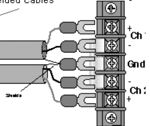
Amplifier Terminal Strip
