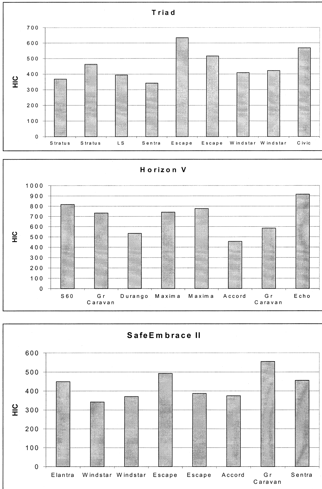
Figure A1: Child Seat Results by Vehicle
