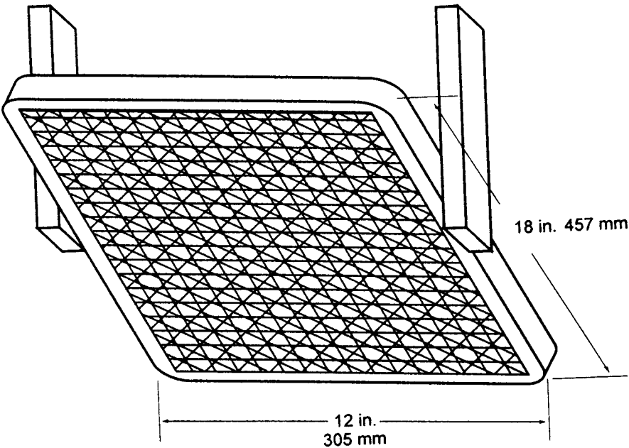
Figure 3a - Air-Propane Radiant Panel
